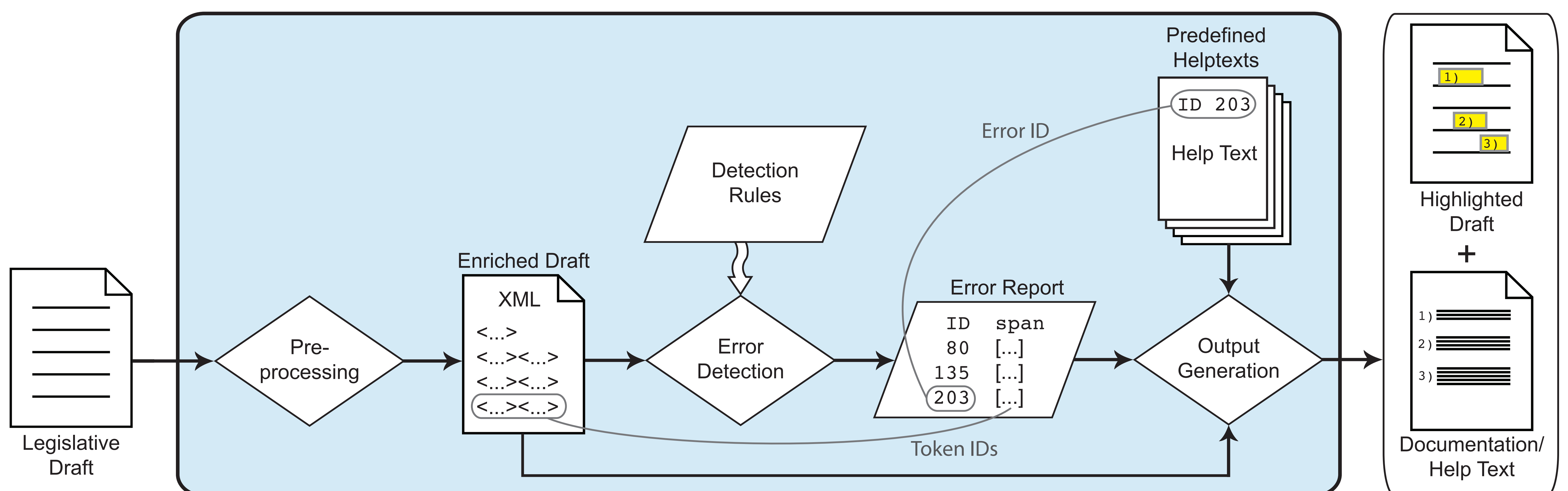
Figure 2: Architecture of the style checker.
