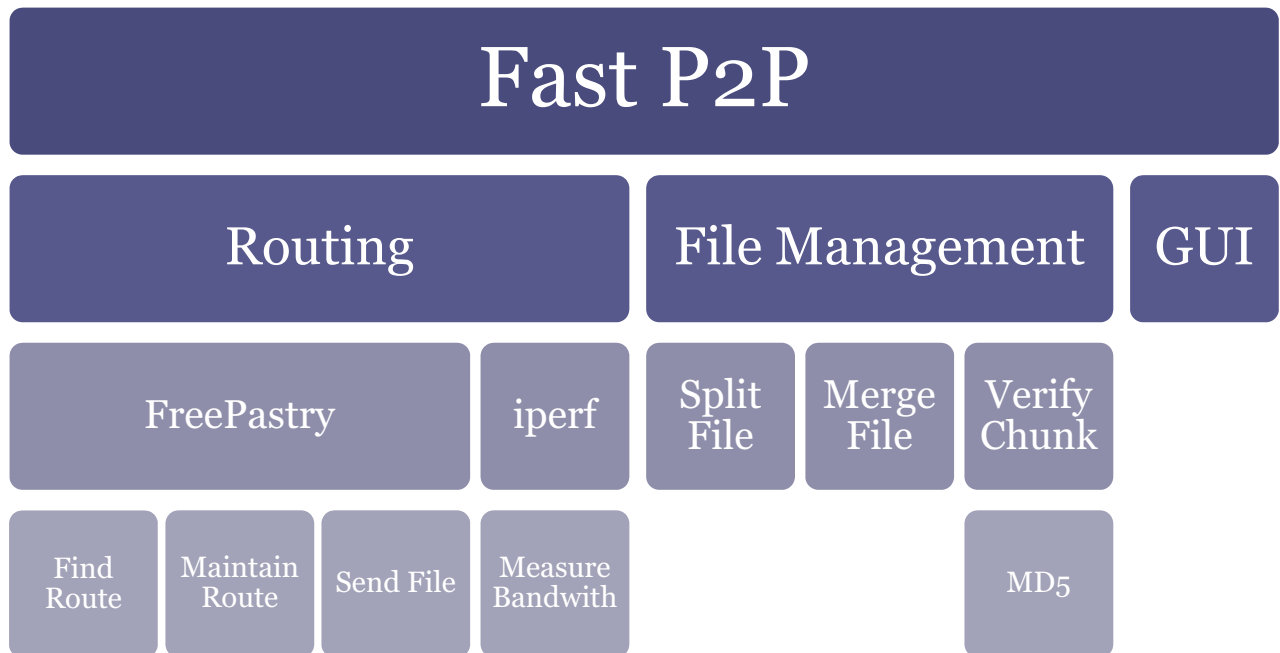
FastP2P architecture
