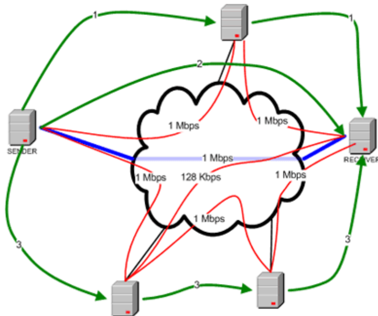
Figure 3: Testbed network topology
